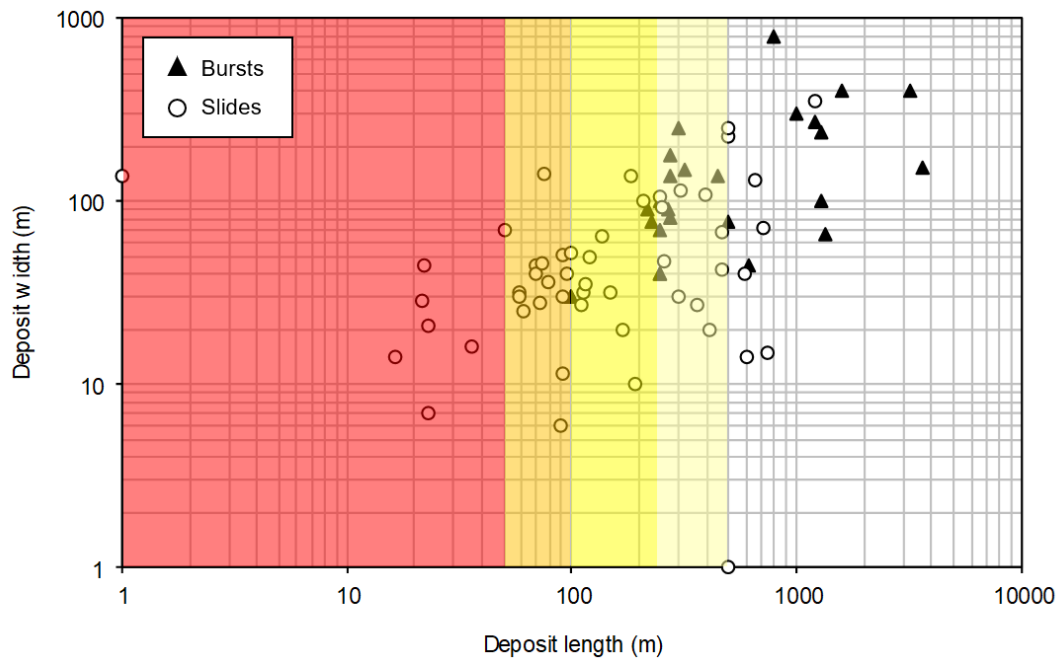
Plate 5.1 Runout distances for published peat landslides (after Mills, 2002), colours on the plot correspond to runout pathway zones on Figure 8.4.10
