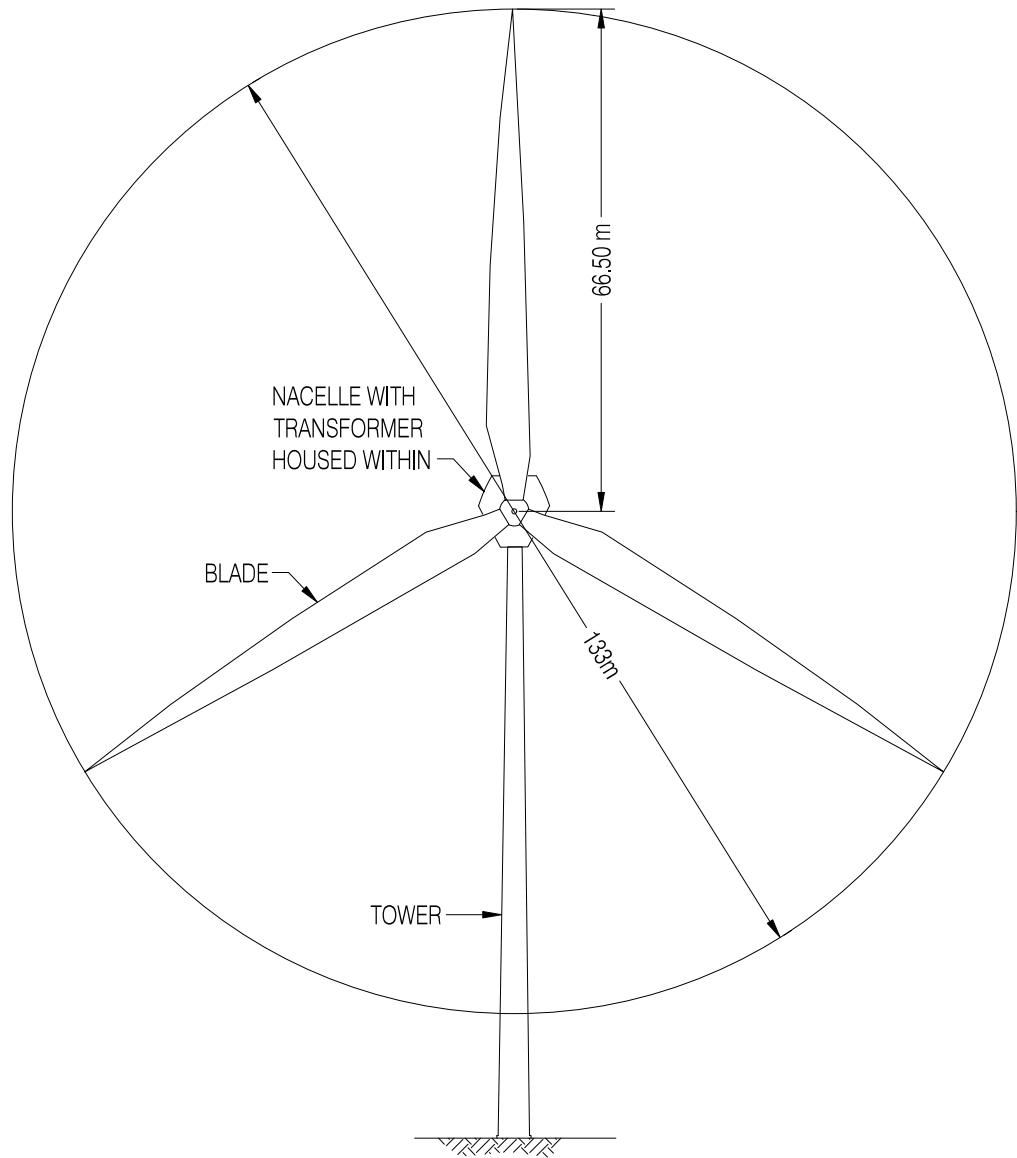
FRONT ELEVATION SCALE 1:1000
