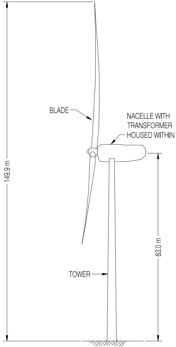
SIDE ELEVATION SCALE 1:1000
